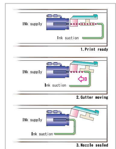
Automatic nozzle capping system.
