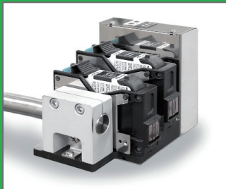
▲ Two lines with one printhead with print height of 25 mm
